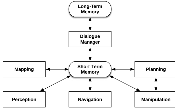
Fig. 1. Software architecture of UNSW@Home
