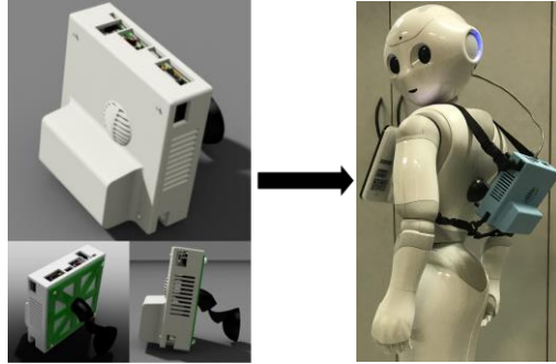
Fig. 4. The Pepper's Backpack is a simple 3D printed enclosure for Nvidia Jetson TK1 with space for a battery. It can be easily attached to Pepper without impairing his movements.
