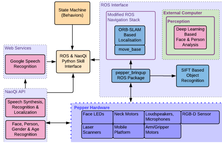
Fig. 5. Pepper main software diagram
