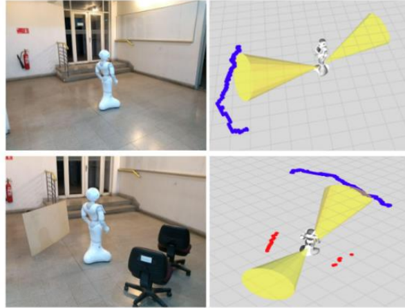
Fig. 1. Pepper's sensors visualization. Blue corresponds to a simulated Laser Scan from depth images. The sonars are represented by the yellow cones. The LIDAR (red) does not register measurements in the first scenario because the walls are out of range. In the second scenario, the readings for a wall and a pair of chairs are very similar.
