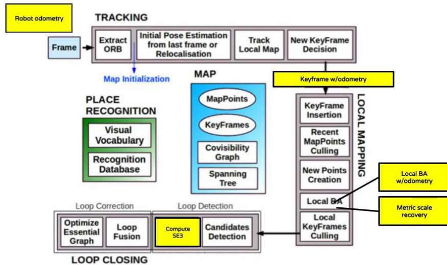
Fig. 2. ORB-SLAM modified software diagram. The yellow blocks correspond to the modifications. First, odometry information is added as an input together with the frames. Second, all the Keyframes have an odometry measurement associated.
