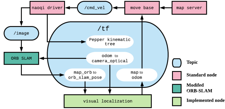
Fig. 3. Software diagram for the localization and navigation system. ORB-SLAM is connected to the standard ROS Navigation System.
