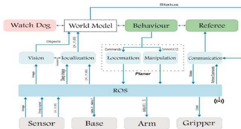
Fig. 5. Software architecture
