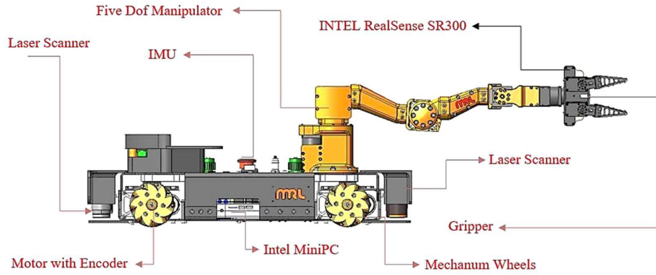
Fig. 1. MRL@Work Robot
