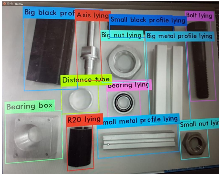
Fig. 2. 2D object detection using Yolo.
