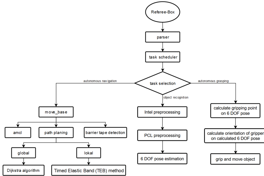
Fig. 2. Simplified representation of the main software components and their interactions
