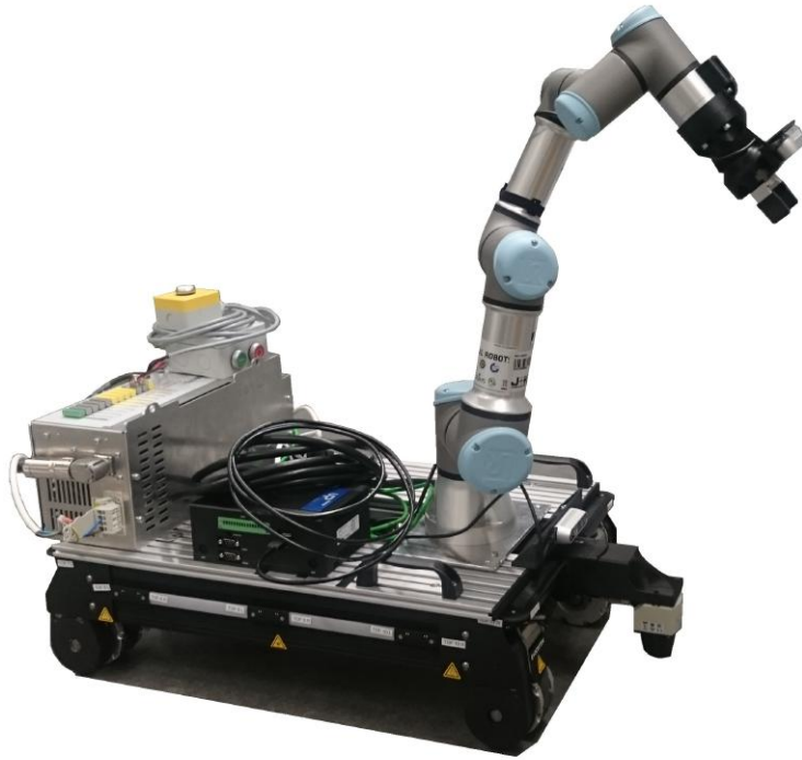
Fig. 1. The current robot with the Evocortex as base, the UR3e, and the Hand-e
