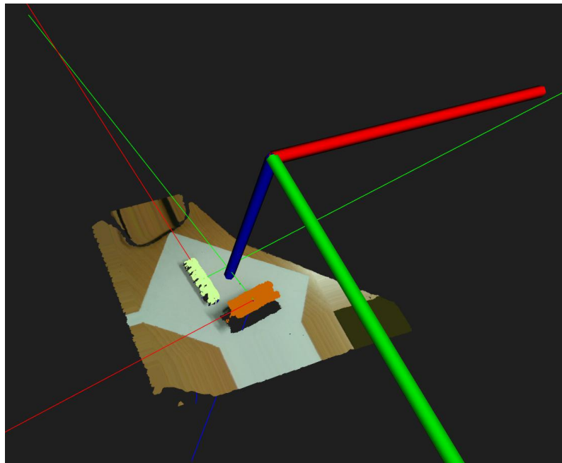
Fig. 3. 3D vision
