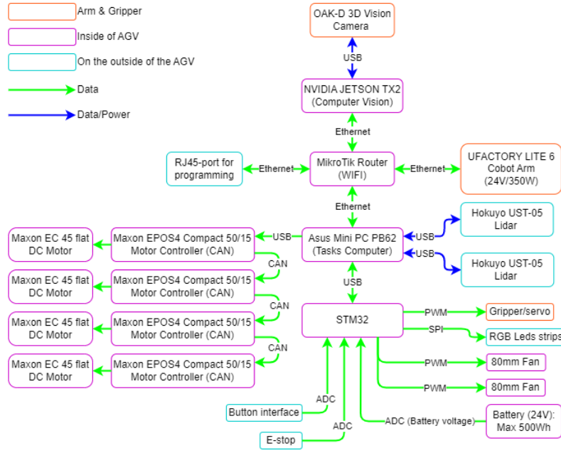
Fig. 2. The hardware diagram from SLICK.
