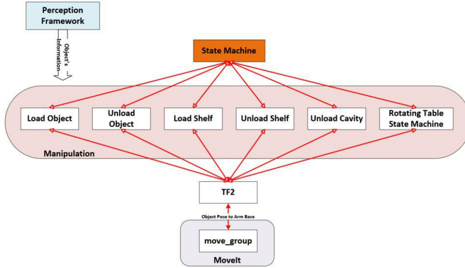
Fig. 9. Manipulation Architecture
