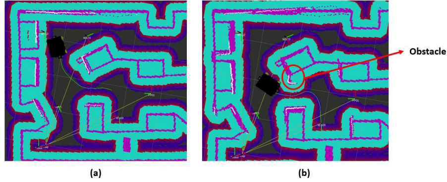
Fig. 6. (a) Normal Trajectory (b) Obstacle Avoidance Trajectory
