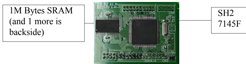
Fig. 7. SH2 CPU board
