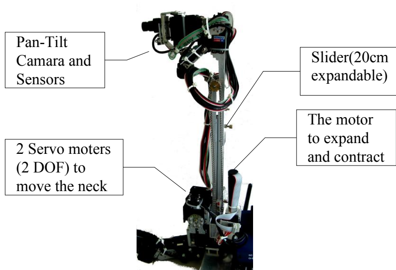
Fig. 9. The neck which can expand and contract
