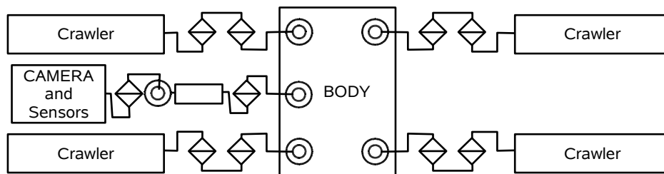
Fig. 6. DOF diagrams of 4Legs
