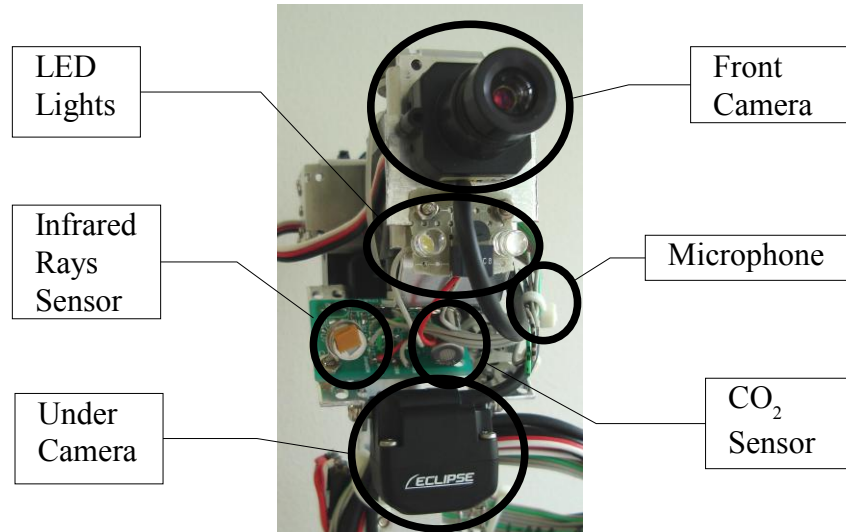
Fig. 4. Camera and Microphone and Infrared rays sensor and CO 2 sensor
