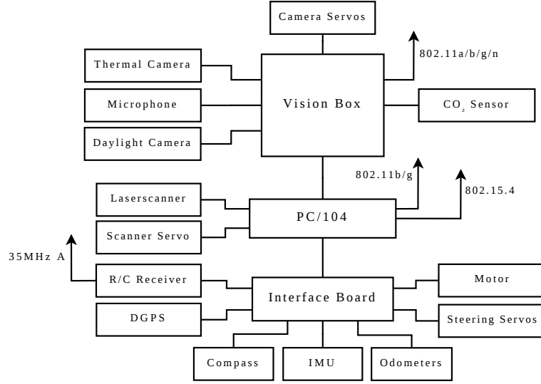
Fig. 4. Structure of hardware components
