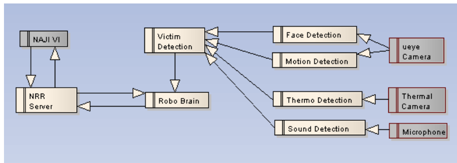
Fig. 7. overview of autonomous robot.
