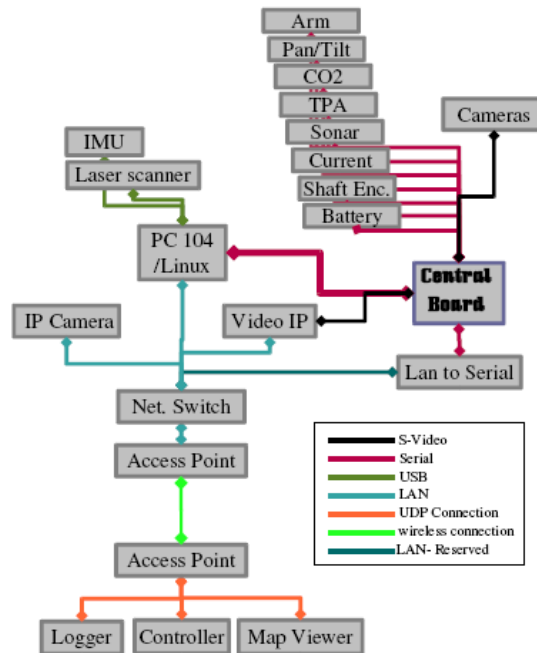
Fig. 8. high level overview of semi-autonomous robots
