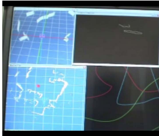
Fig. 7 human-robot interface for KAMUI. Up-left; wall image based on laser range-finder. Up-right; the area enclosed with white line is high temperature area by thermal camera. Low-left; generated 2D map of the environment.
