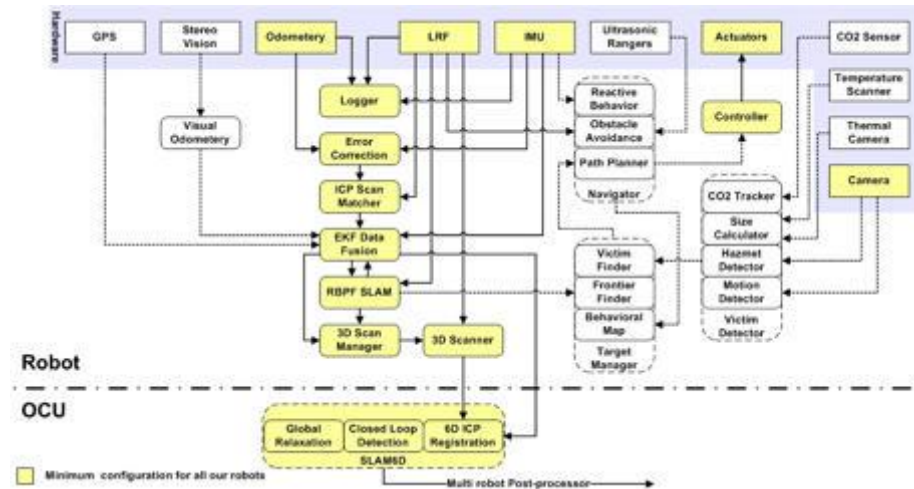
Fig. 3. Architecture of our software (Yellow boxes denote minimum requirements for tele-operation)
