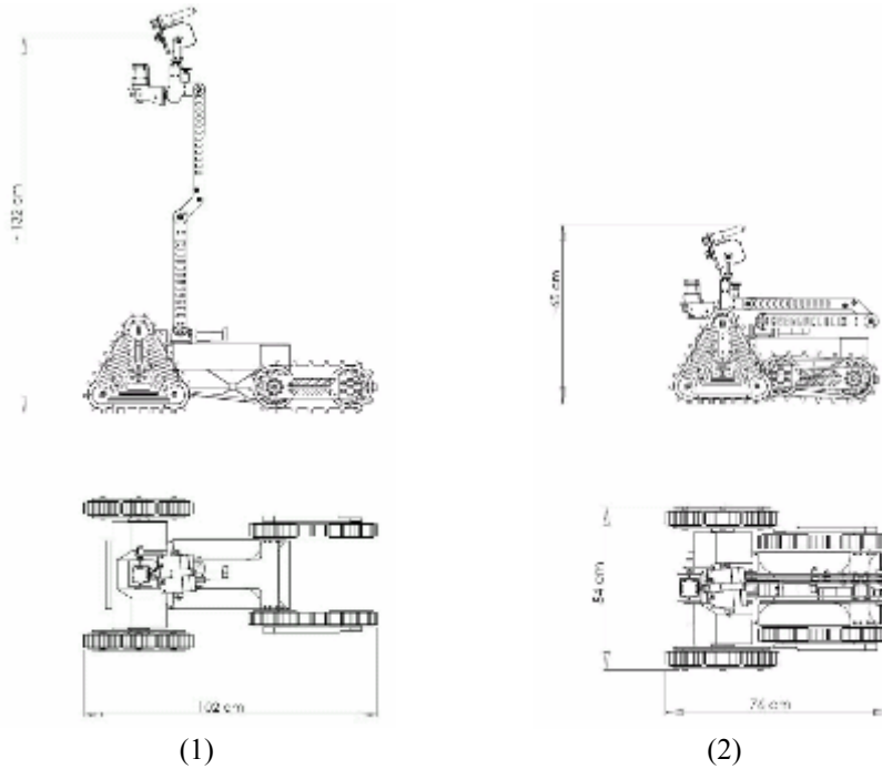
Fig. 8. Overall dimensions of BETA: (1) extended, (2) stowed configurations
