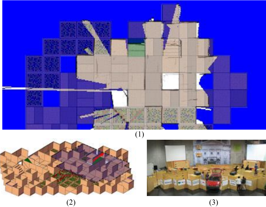
Fig. 5. An example of OG mapping by our tele-operated robot in RC09 (2nd semifinal round): (1) 2D map overlayed with ground truth model (2) 3D model of the arena to generate ground truth map (3) Real arena for comparison with simulated model
