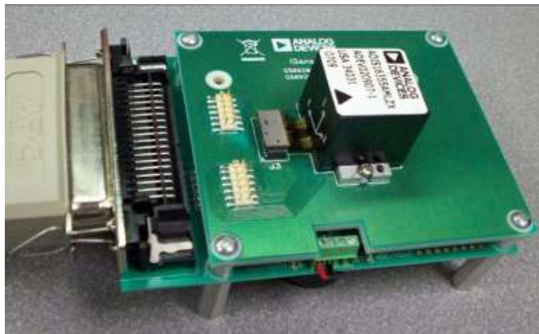
fig 6.2: iSensor based in MEMS 3D level and acceleration [14].
