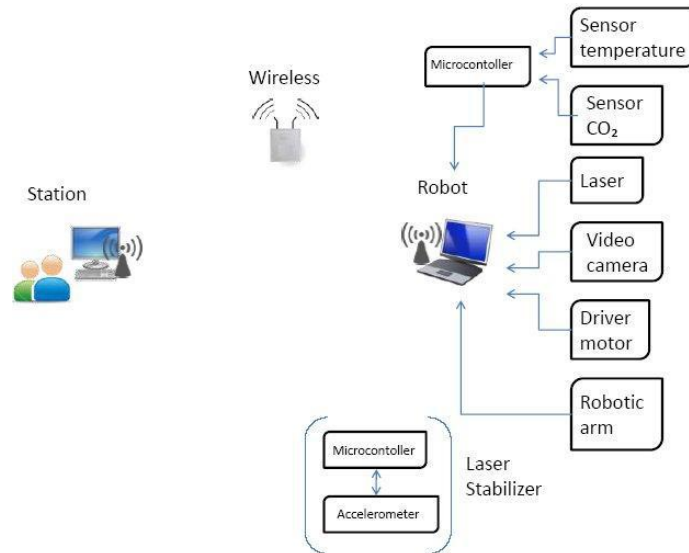
Fig. 1 Block diagram of the rescue robot IXNAMIKI.
