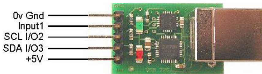
Fig. 4. I2C Connections.
