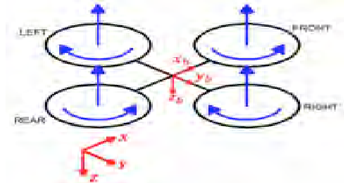
Fig. 14. Quadrotor control and navigation frames
