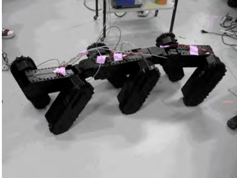
Fig. 2 KOHGA2 (3 bodies and 6 crawler arms)
