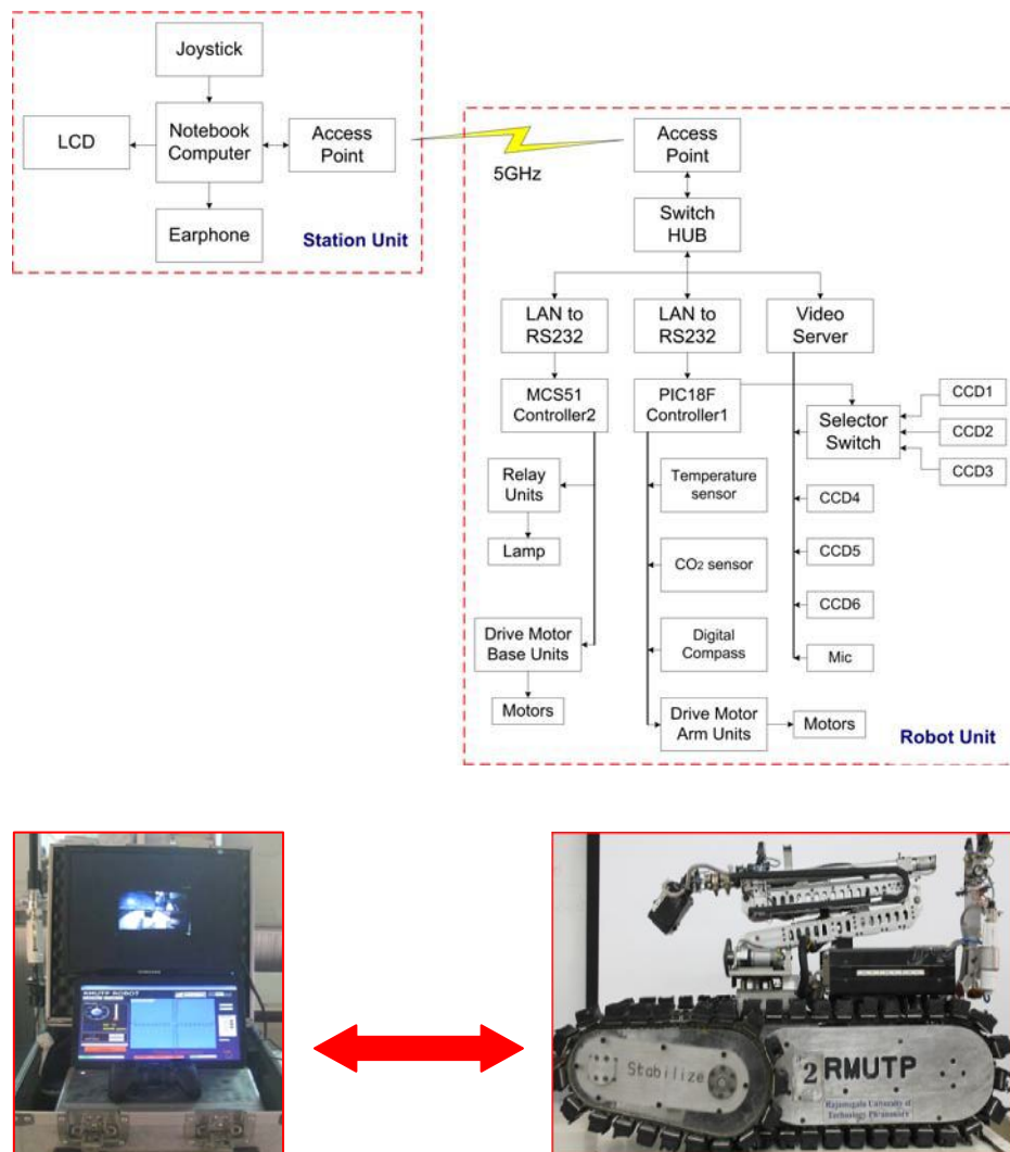
Fig. 3. The control system used by STABILIZE.
