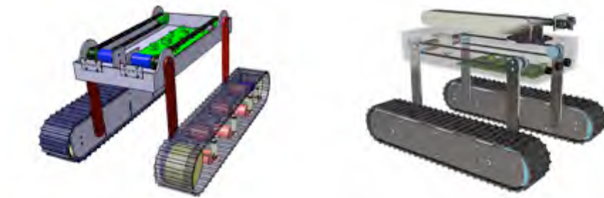
Fig. 4 The internals of the mechanism of the main body and the tracks and a photorealistic view of the robot.
