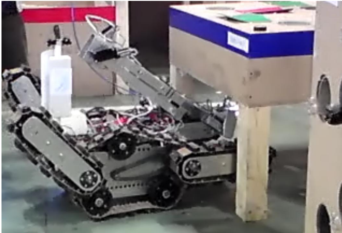
Figure23: Final Assembled of Manual Robot
