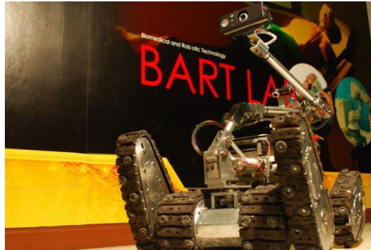
Fig. 1. The TeleOpIII, one of our two tele-operative robots in BART LAB Rescue team. The TeleOpIII employs tracked locomotion system with 4 independent flippers, and equips with an inverse-kinematically controlled manipulator to enhance more ability to search and retrieve better victim information, similar to other robots in [1,2]
