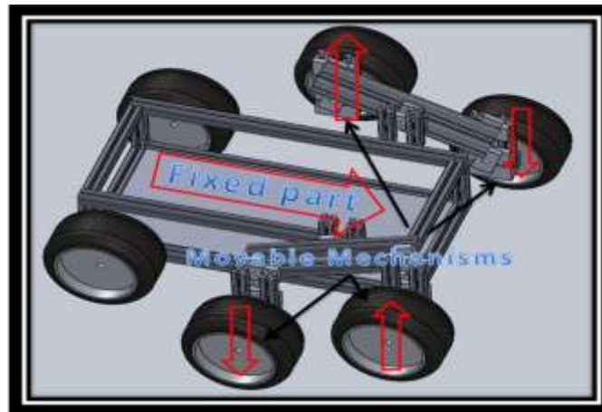
Fig 8.2 Mechanic movement of structural mobile robot
