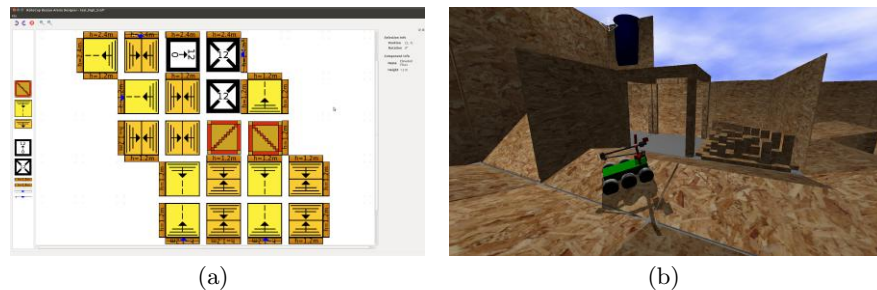
Fig. 7. USAR scenario simulation: (a): Screenshot of the GUI tool for creating USAR scenarios showing an example scenario (b): The same scenario as simulated in gazebo simulation
