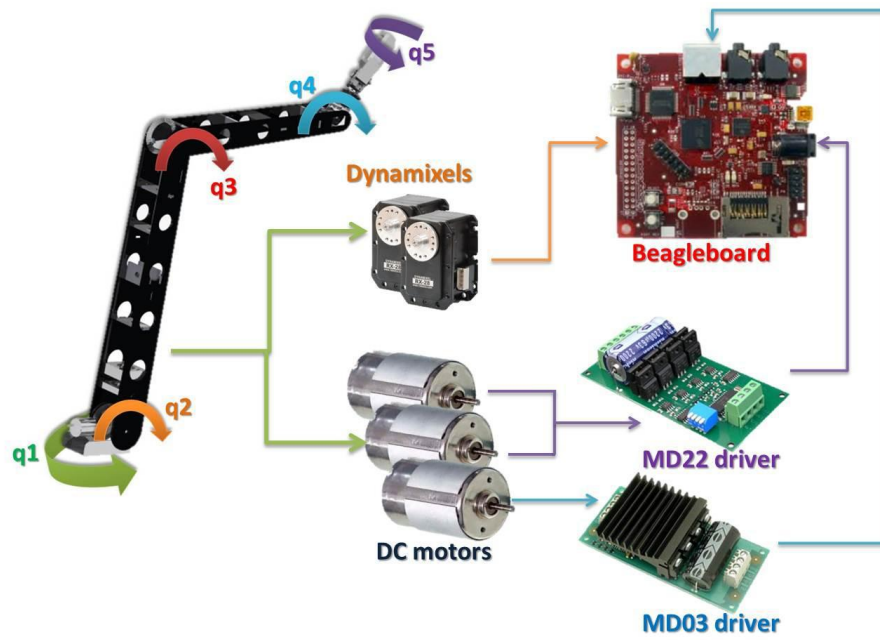
Fig. 10 Manipulator mode's architecture.
