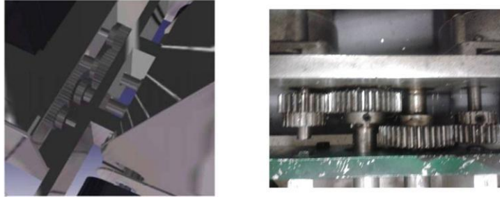
Fig. 25 First reduction stage with spur gears.
