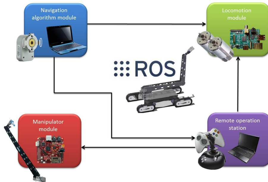
Fig. 7 Xaac's architecture.
