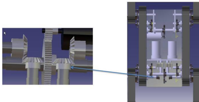
Fig. 29 Second stage, Xaac's transmission of locomotion
