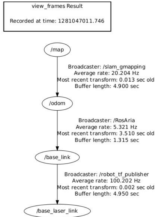
Fig. 15 Tree transformation in ROS.
