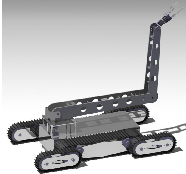
Fig. 4 Render of the design for the new robotic platform (Xaac).
