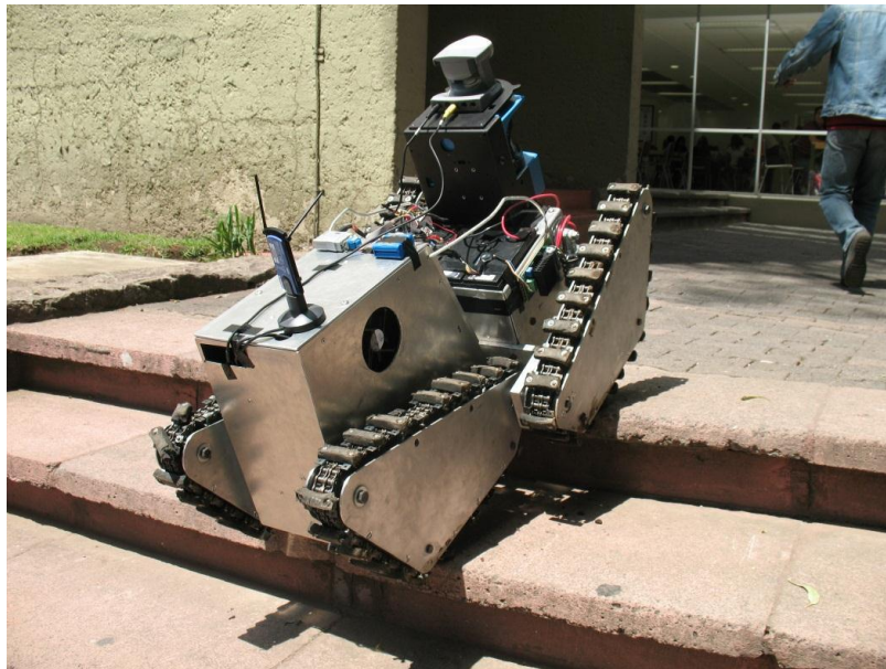
Fig. 2 Kaul rescue robot.
