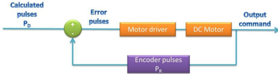
Fig. 11 Closed loop control framework for manipulator's DC motors.
