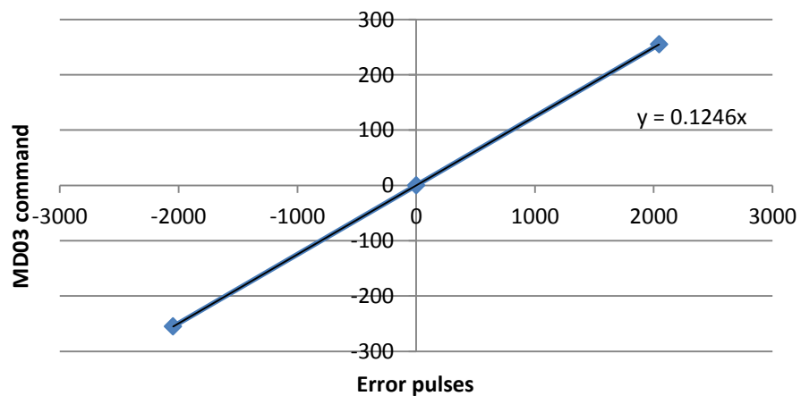
Fig. 13 Linear regression used to calculate MD03 drive's commands
