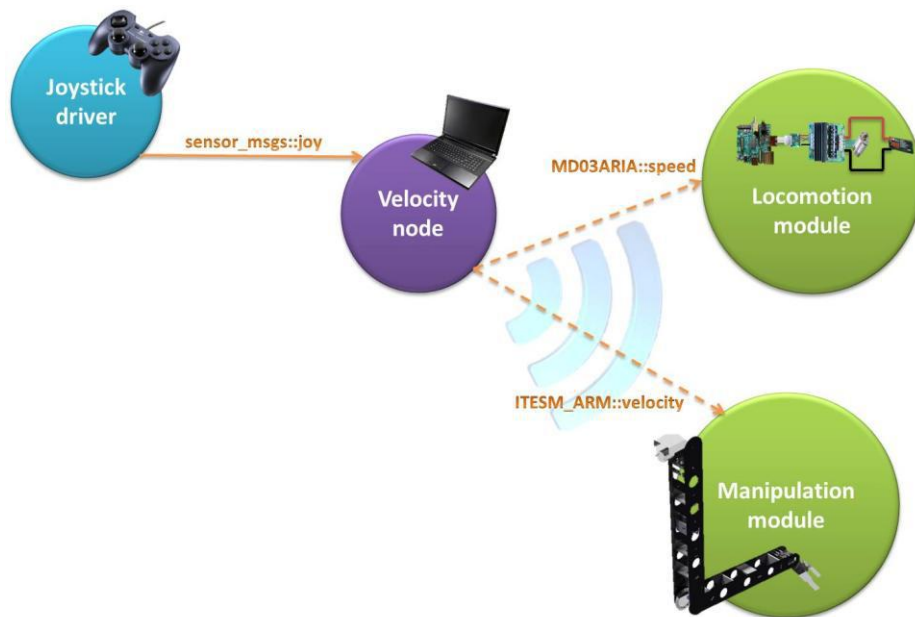
Fig. 9 Remote operation station's architecture.
