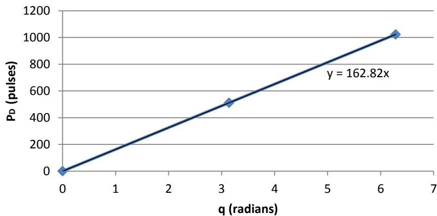
Fig. 12 Linear regression used to calculate the desired pulses.
