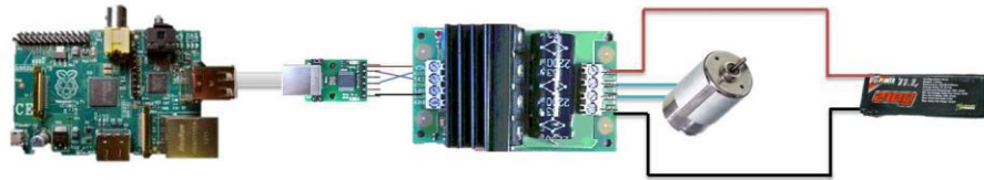
Fig. 8 I 2 C communication structure.
