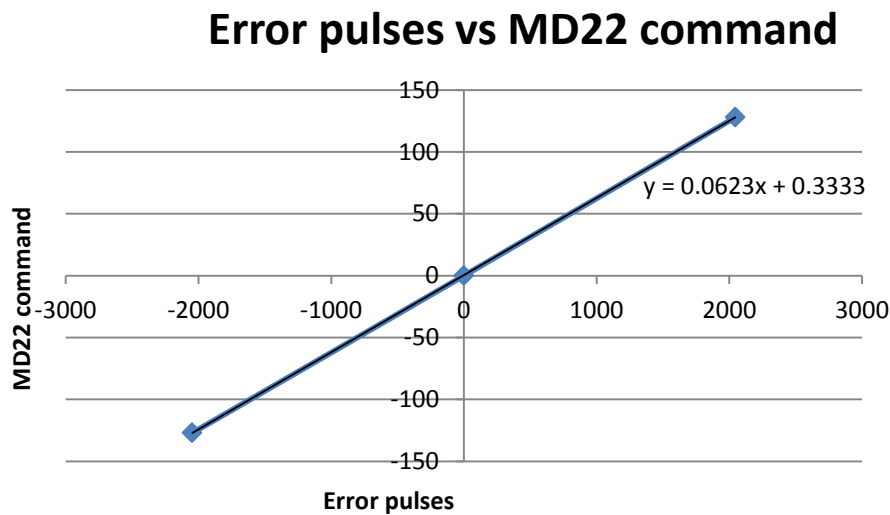
Fig. 14 Linear regression used to calculate MD22 drive's commands
