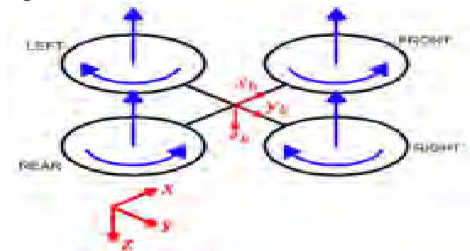
Fig. 16. Quadrotor control and navigation frames
