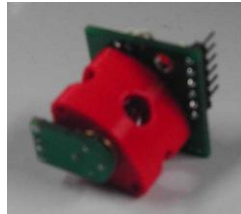
Fig. 6. RKRS custom CO 2 sensor with Heimann gas detection element.
