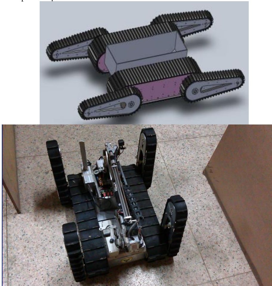
Fig. 15. Tele-operative robot
