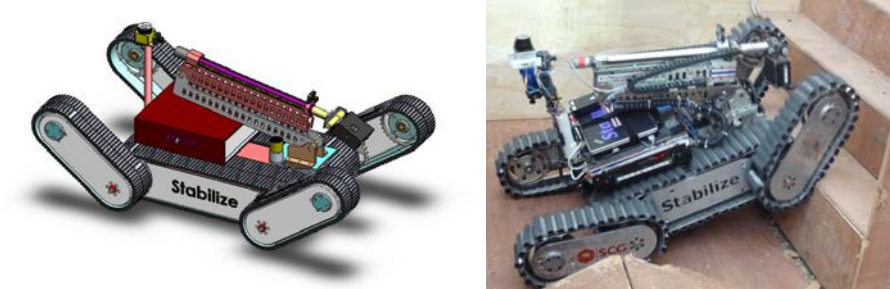
Figure 12. STABILIZE 's tele-operative robot.
