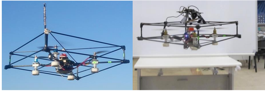
Fig. 12. QUADVIN-Flyer-I
