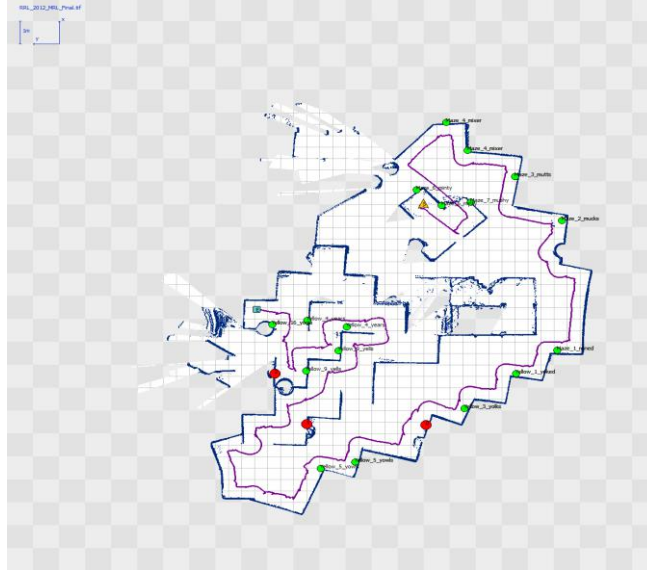
Fig. 15. Illustrates the generated map by MRL autonomous robot at the final mission of RoboCup 2012. The robot exploration started from middle of the arena and autonomously explored the arena and it was capable of finding 3 victims (red markers), and 17 QR codes (green markers).
