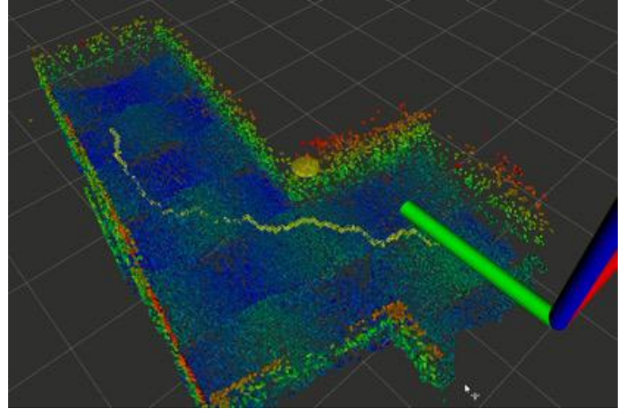
Fig. 3. Path planned on-top of our 3D map.
