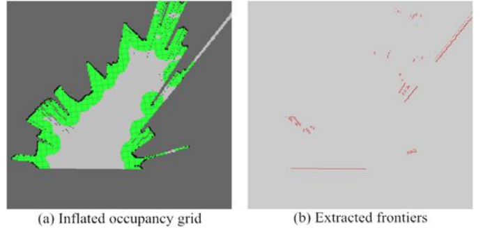
Fig. 6. Occupancy grid with inflated obstacles and the extracted frontier. In (a), green areas are the inflated obstacles.
