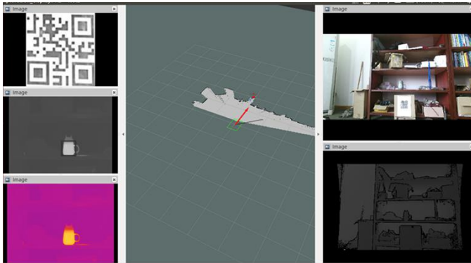
Fig. 10. The result of victim detection and localization, where the found victim is marked by red dot in the map.
