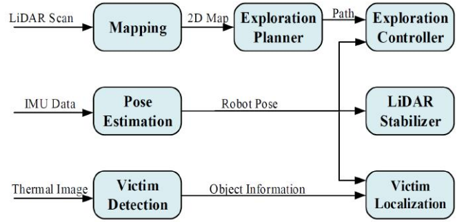
Fig. 2. The software architecture based on ROS. ROS nodes are represented by rectangles, topics by arrow-headed and services by diamond-headed lines. Services are originated at the service caller.
