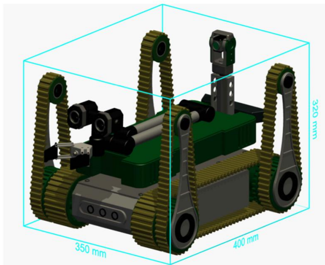
Fig. 7. Dimentions of the robot
