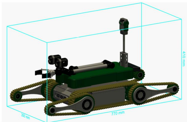
Fig. 8. Dimentions of the robot with flippers extended
