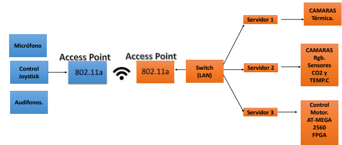
Fig. 4. Communication structure
