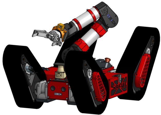
Fig. 3. Markhor Robot CAD Drawing
