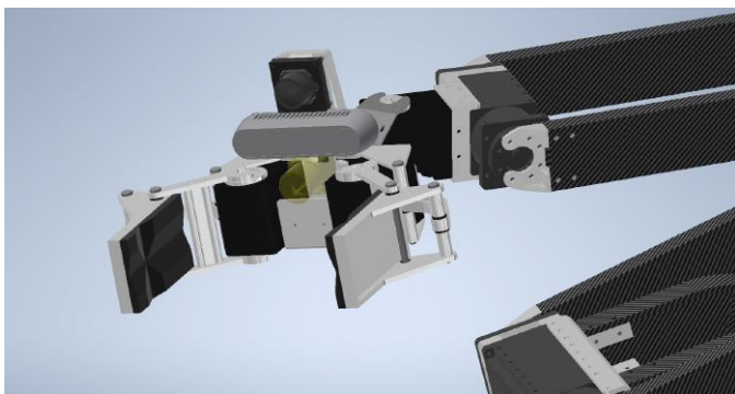
Fig. 3. The hand has 3-DoF wrist and fingers actuated with parallel-link mechanism. The gripper is jamming gripper created by Tohoku Univ.
