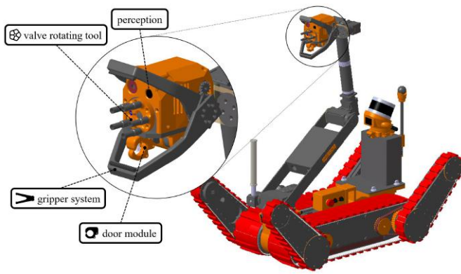
Fig. 6. HURRICAN - CAD drawing of the new tracked rescue robot for Team DYNAMICS
