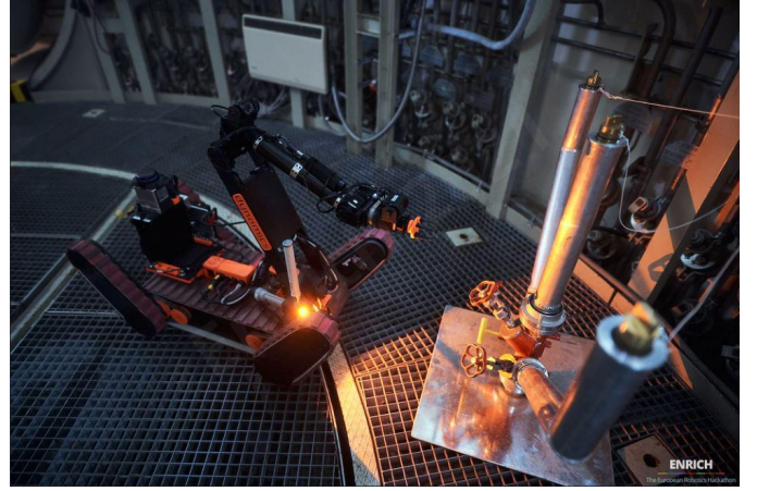
Fig. 15. Robot exploration in a real nuclear facility
