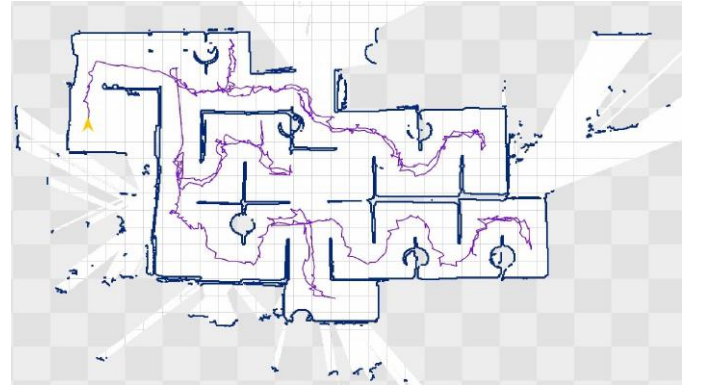
Fig. 9. The automatic map generated by iRAP ROBOT in the final round of the world RoboCup 2019 competition.
