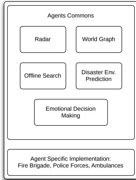
Fig. 1. Impossibles Software Architecture
