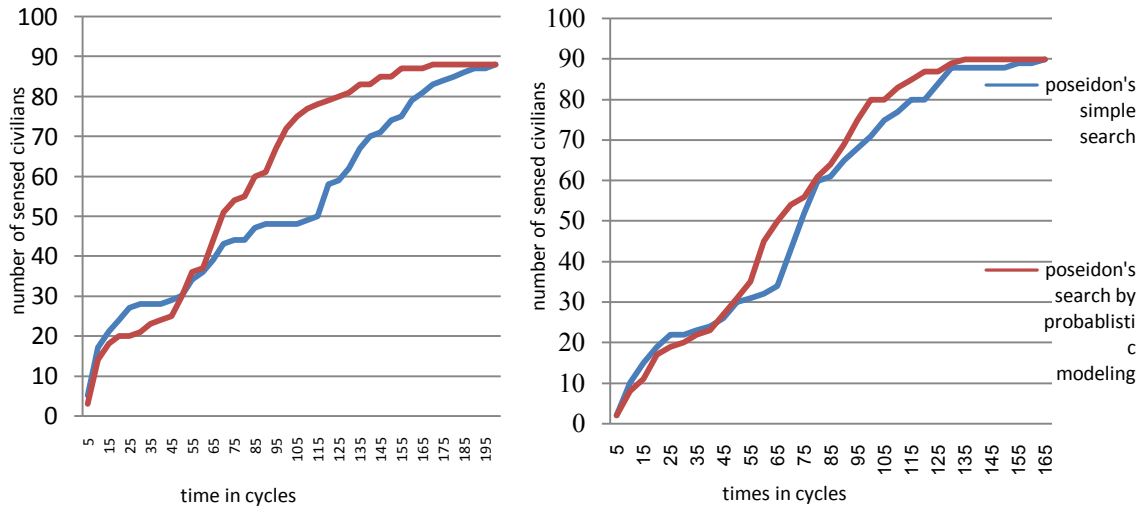
Fig.2. In the right diagram, civilian distribution is steadier. Number of each diagrams, have been gained by running over 10 times of two versions.
