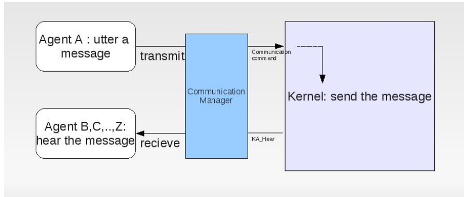
Fig. 2. The communication layer for the agents
