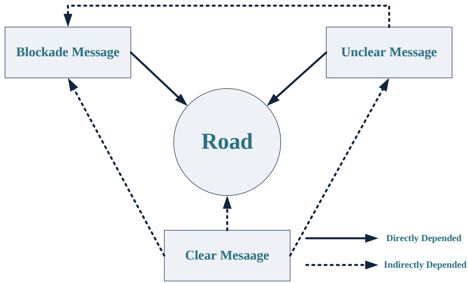
Fig. 8. Relationship among Block, Unclear and Clear Message
