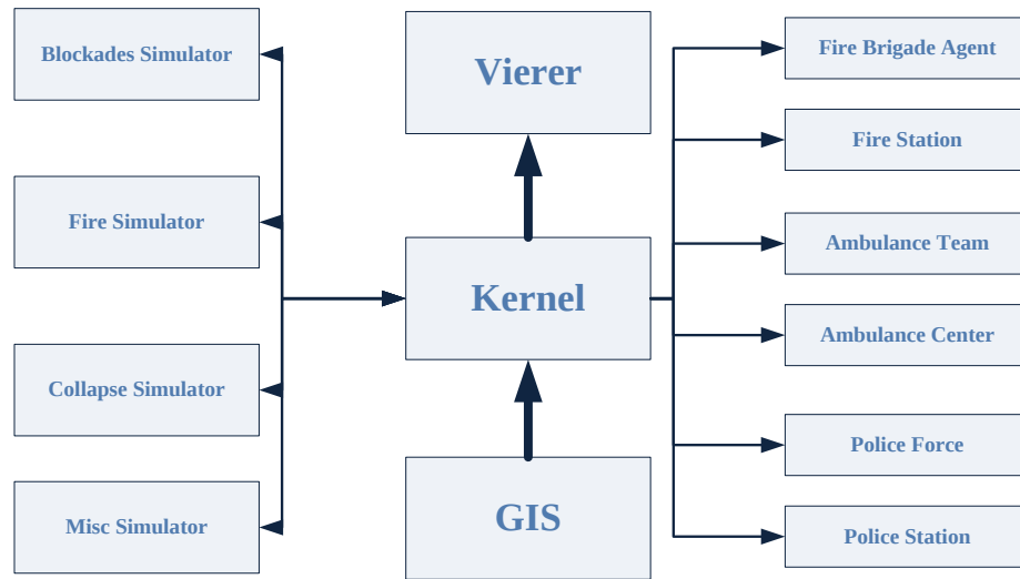
Fig.2. Structure of RCRSS
