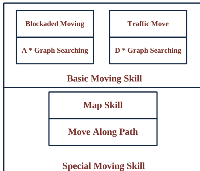
Fig.7. An Overview of Moving Skill
