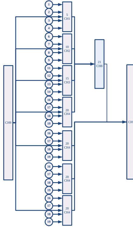
Fig.6. Close loop communication model without centers
