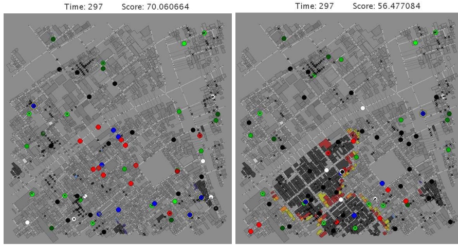
Fig. 2. MinERS fire agents (left) and sample agents (right) on Kobe Large, with 12 fire brigade agents and blockages enabled
