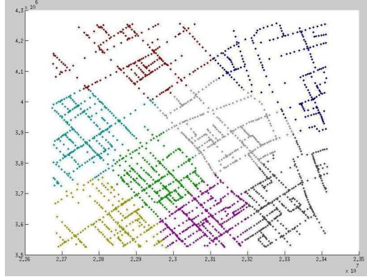
Fig. 1. Kobe Large Map with roads divided into 8 clusters. Roads of the same color belong to the same cluster.
