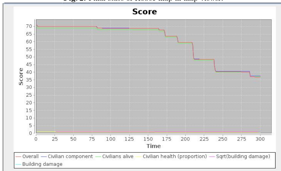
Fig. 3. Final score of Kobe1 map in score chart.
