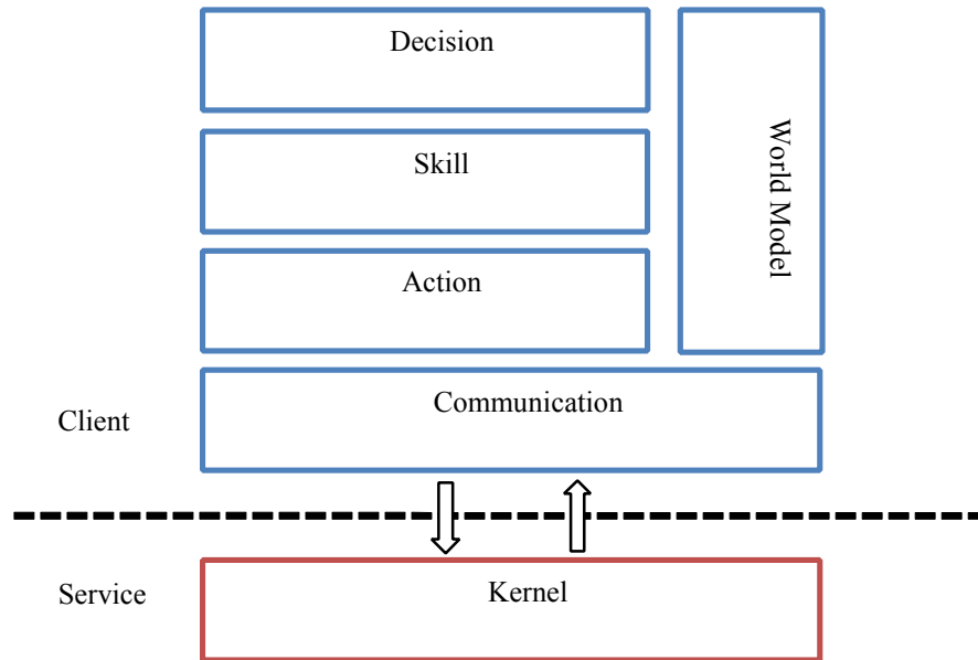
Fig.3. Software Architecture
