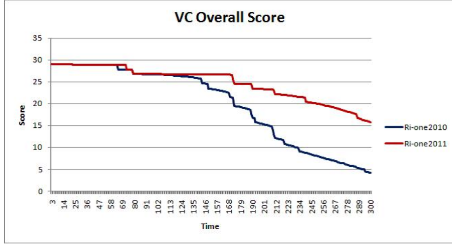
Fig. 4. Overall score
