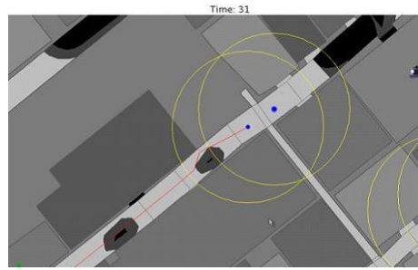
Fig. 1. Blockades' shapes
