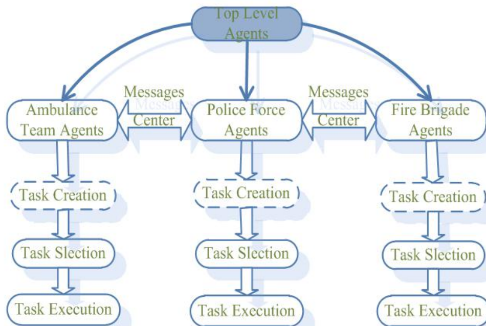
Figure 2 Module Structure of SEU_RedSun
