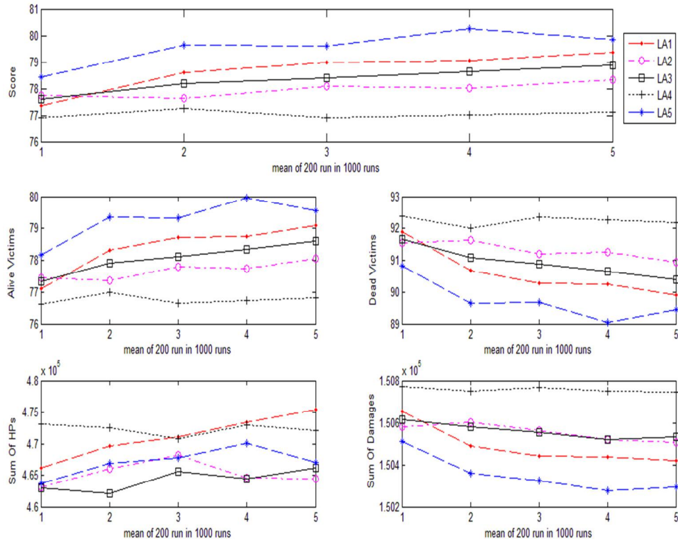
Fig. 3 Learning processes with different parameters
