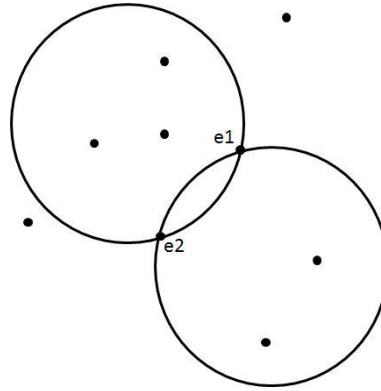
Fig. 3. A circle by two specific points
