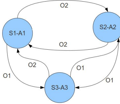
Fig. 2. An Example Finite State Controller
