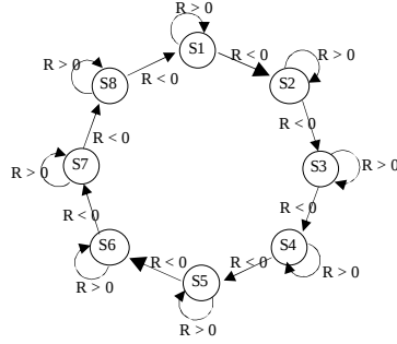
Fig. 1. Learning Automata structure to adjust priorities
